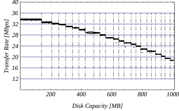
Figure 4: Zone characteristics of the Seagate ST31200W magnetic disk
