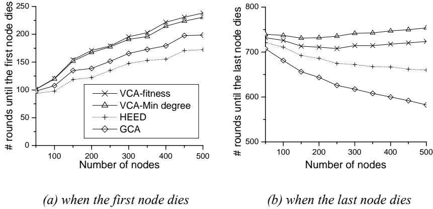
Figure 13. Network lifetime when sensors are mobile
