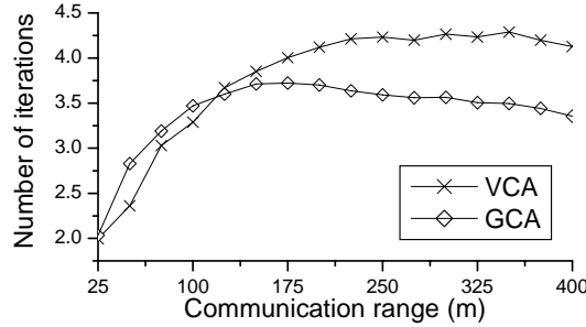
Figure 7. Average number of iterations performed.
