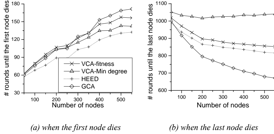
Figure 10. Network lifetime as a function of number of nodes.
