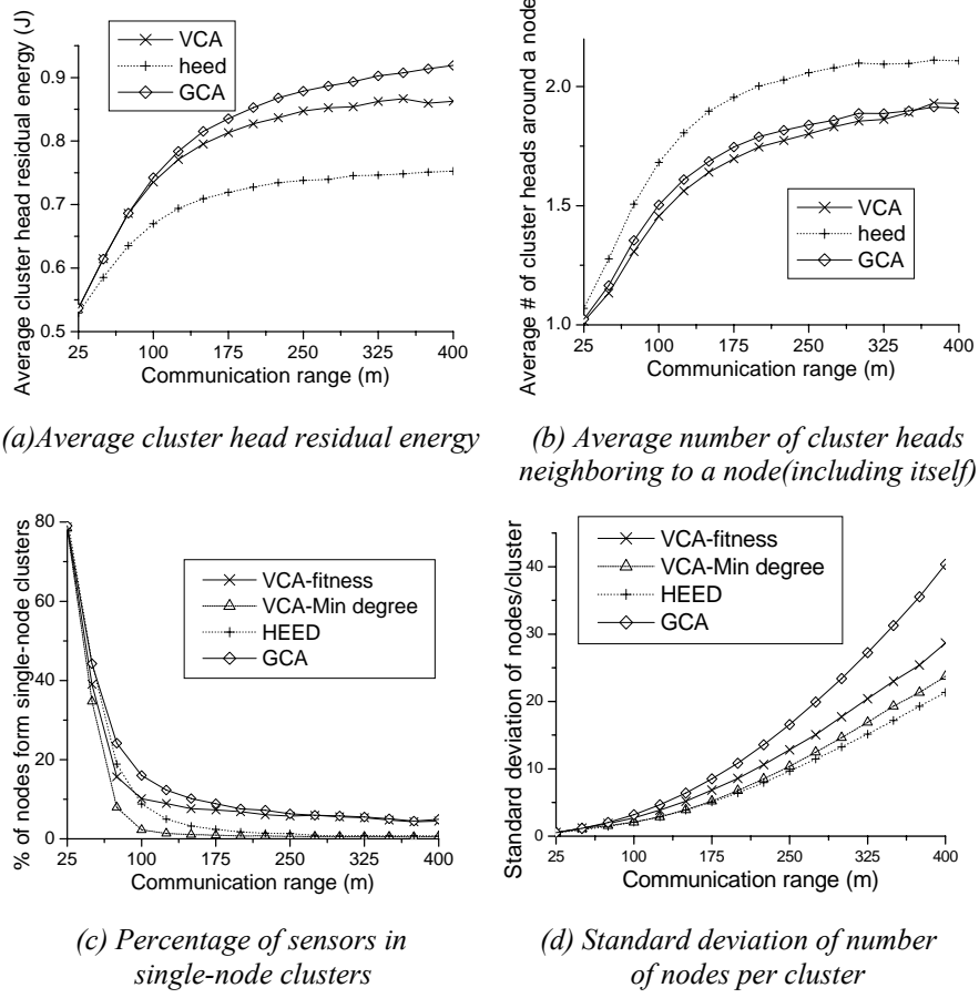
Figure 8. Average cluster properties.
