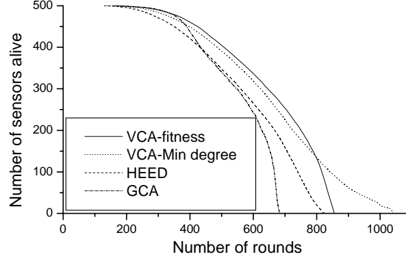
Figure 11. Number of sensors alive when running the protocol continuously for a 500-node network.
