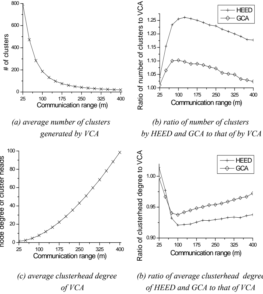
Figure 6. Comparison of number of clusters and clusterhead degree as a function of the radius.
