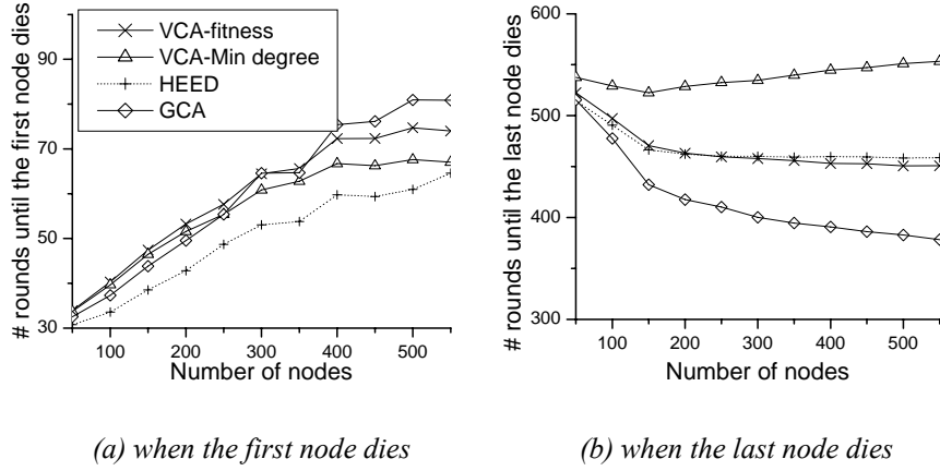
Figure 12. Network lifetime when the network operation time is increased to 20 TDMA frames
