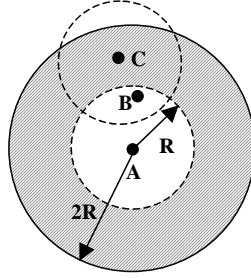
Figure 5. Non-neighboring cluster heads around a sensor.
