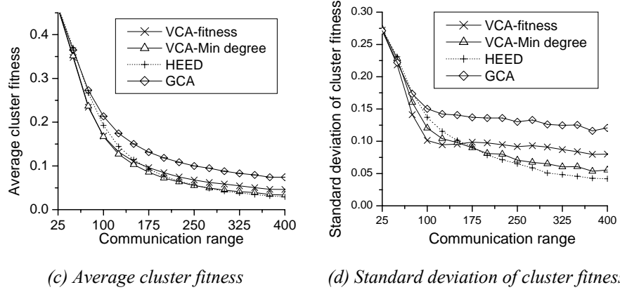
Figure 9. Average cluster fitness.
